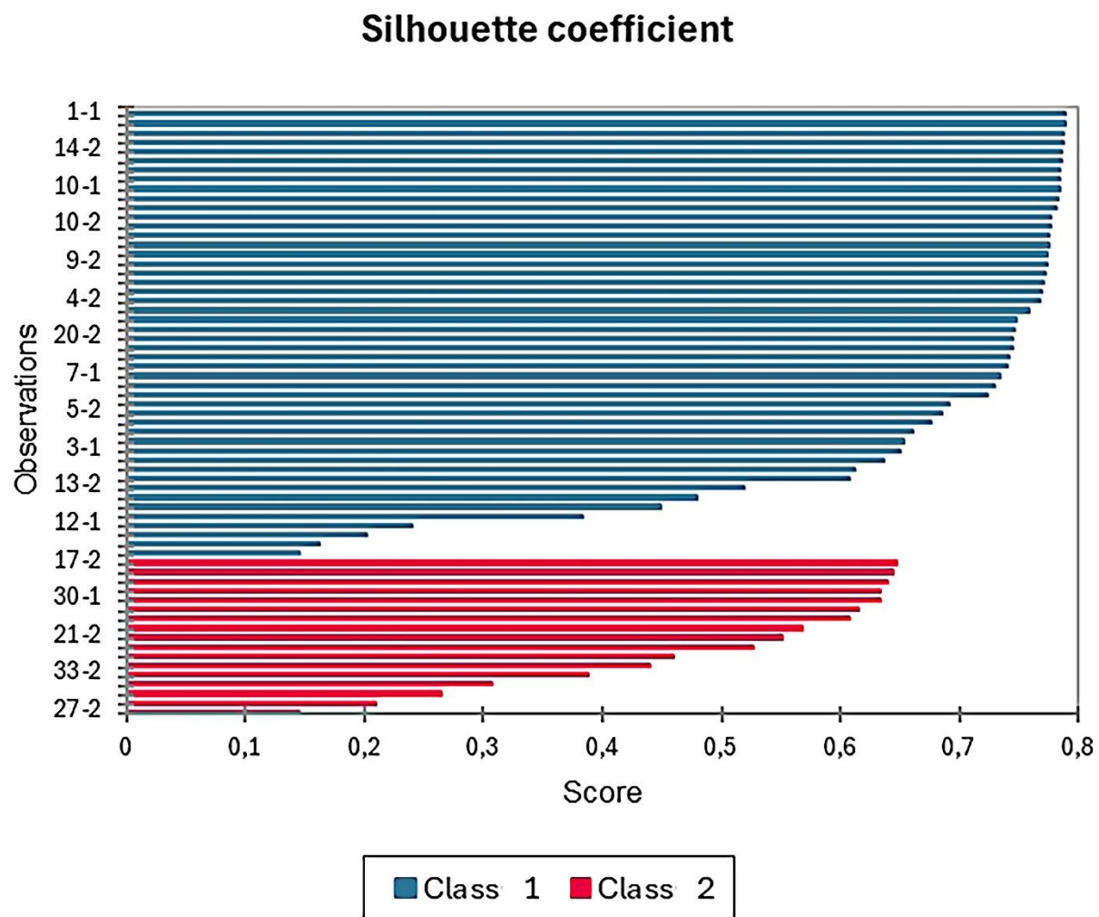
Figure S1: Classification of canters using the k-means method based on judges' scores ( A_1 + A_2 ).
